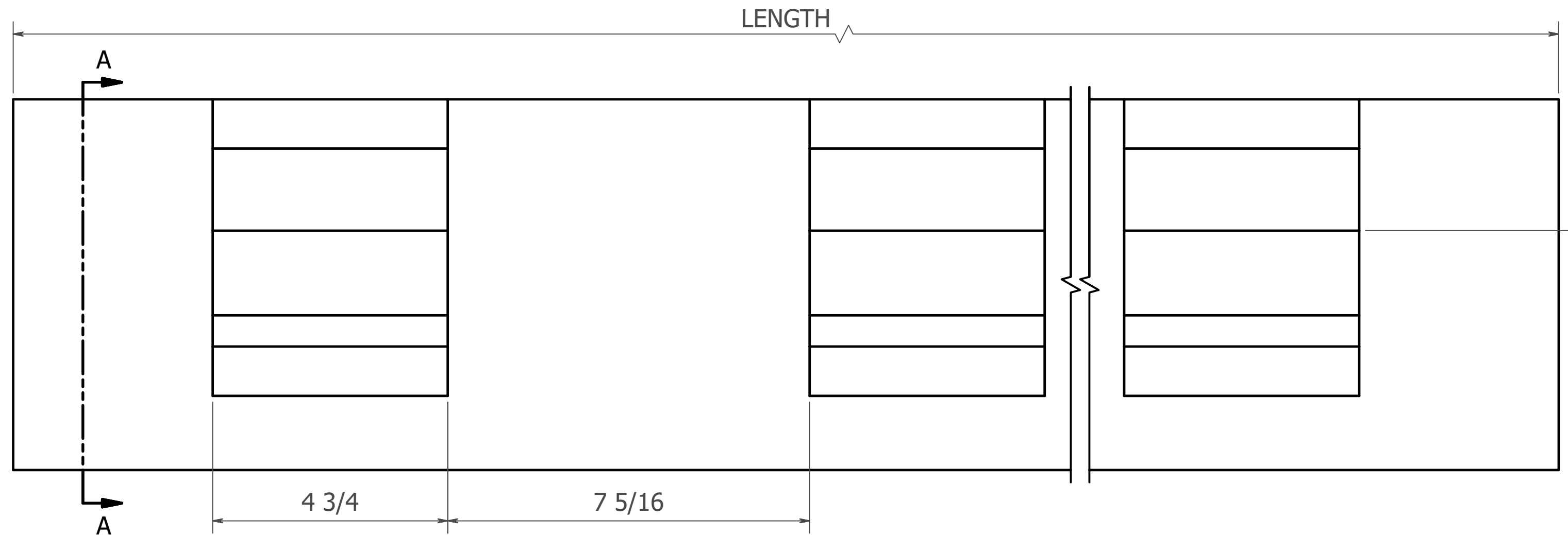
FRONT SCALE 1 / 2
