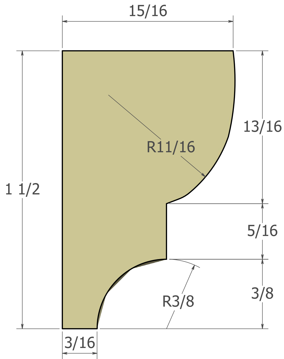
PROFILE SCALE 4 : 1
