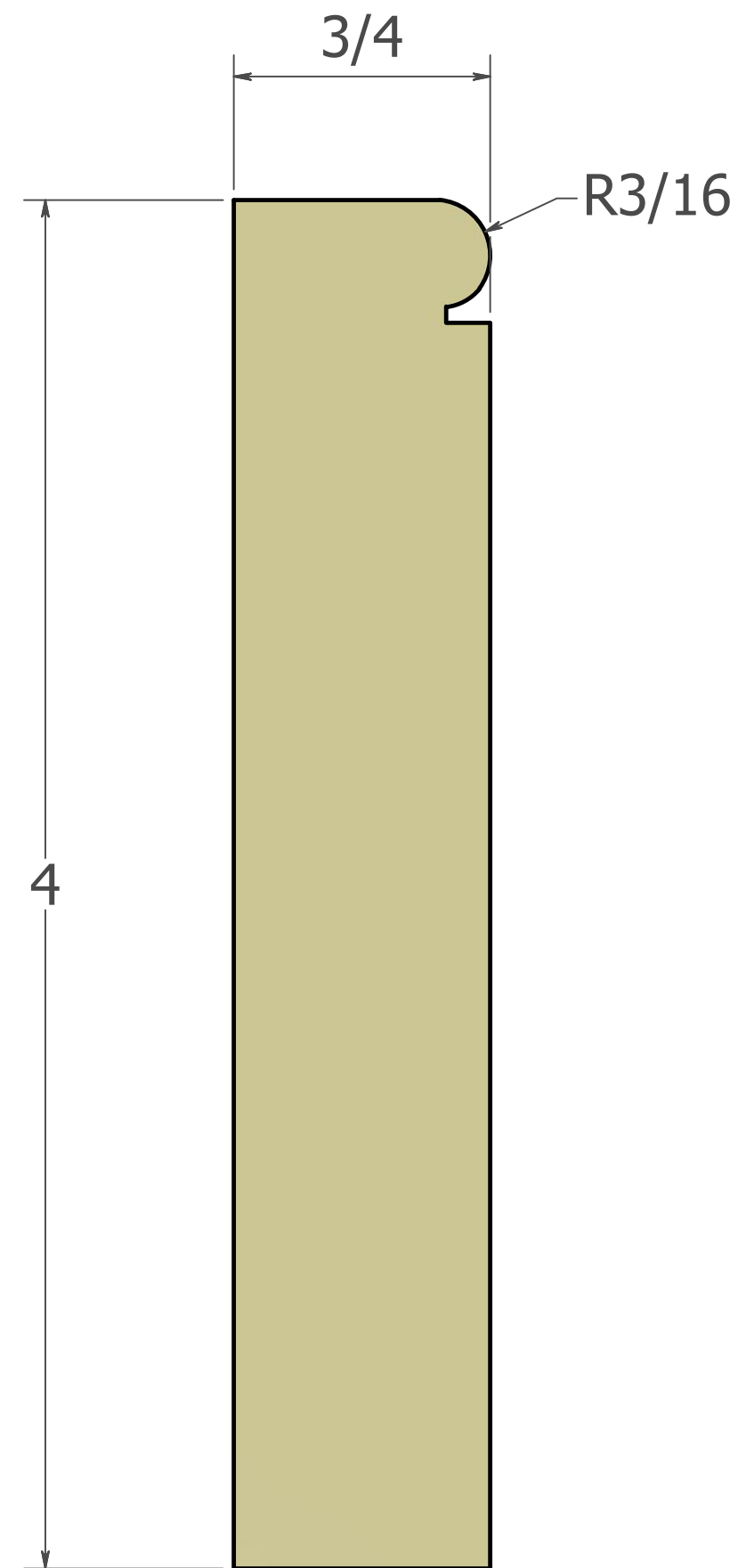
PROFILE SCALE 2 : 1
