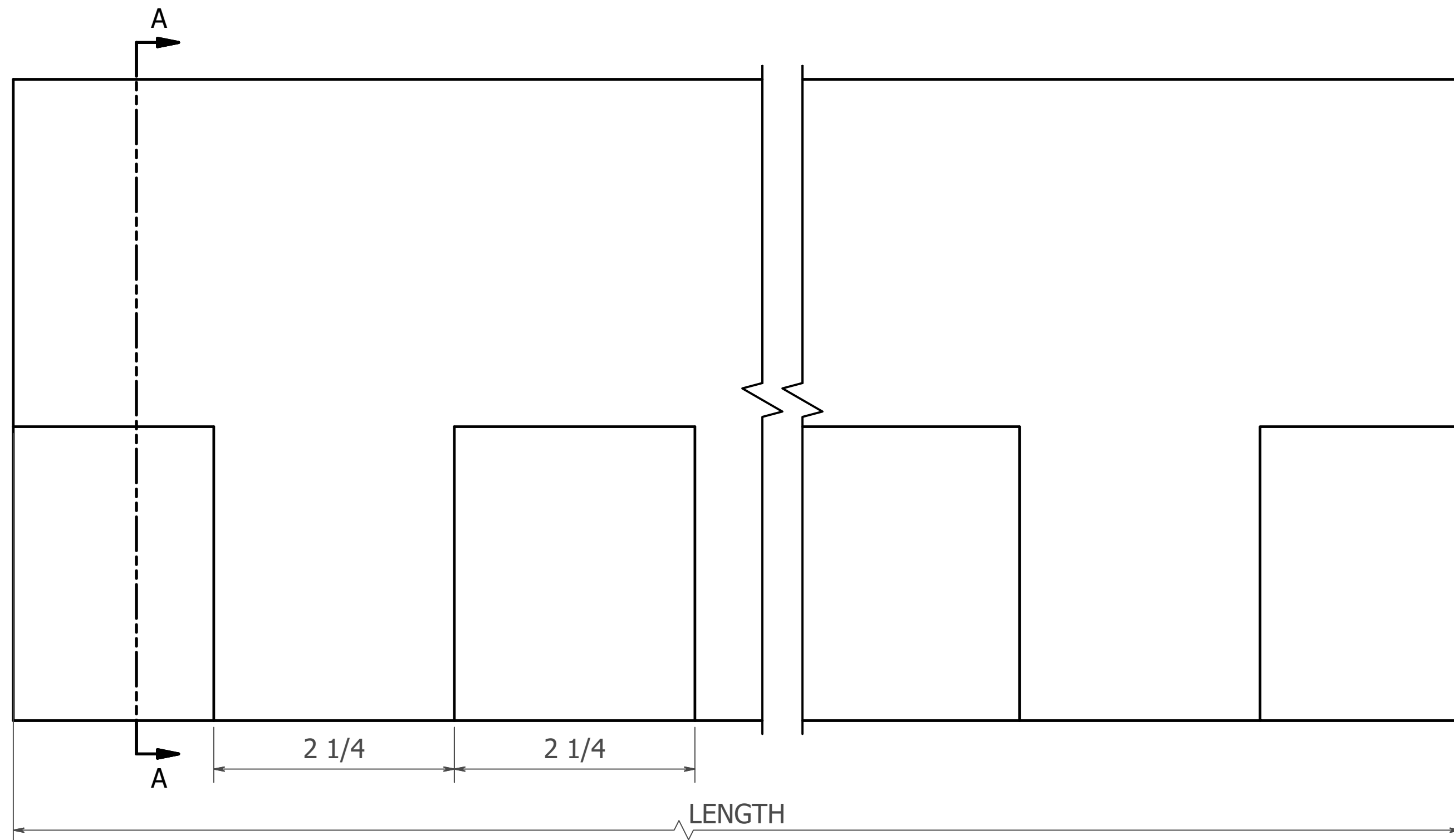
PROFILE SCALE 1 : 1
