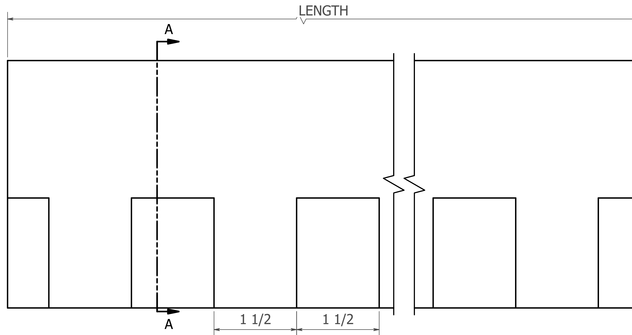
PROFILE SCALE 1 : 1
