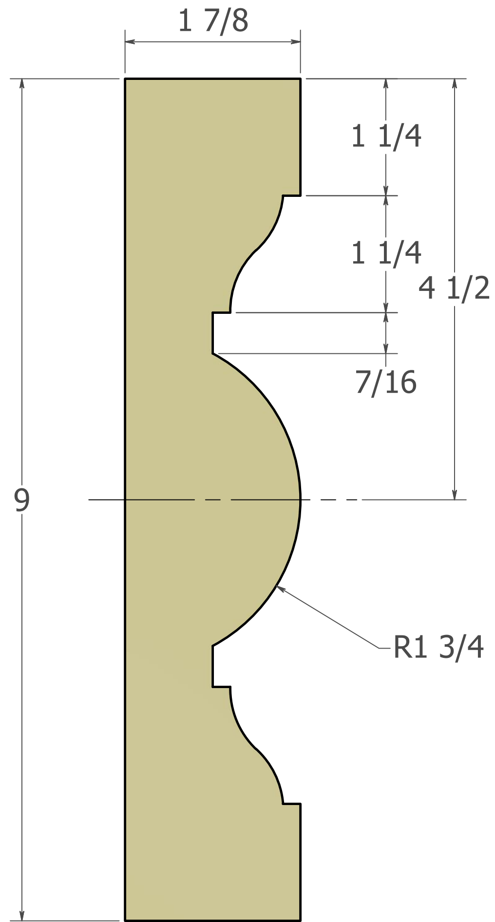
PROFILE SCALE 1 : 1
