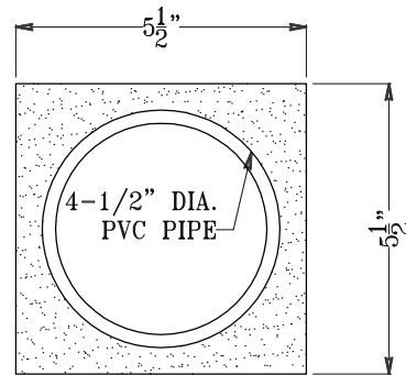
SECTION - FLAT NEWEL POST ARCH. REF. N.A. SCALE 3"=1'0"
