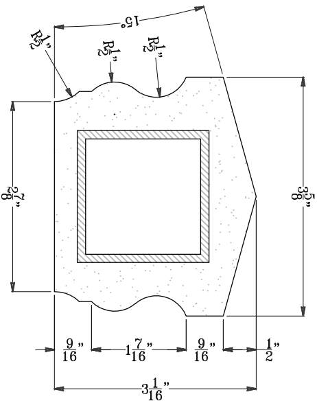
END VIEW - TOP RAIL
