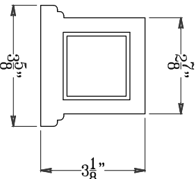
END VIEW - BOTTOM RAIL ARCH. REF. N.A. SCALE 3"=1'0"
