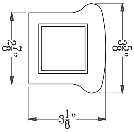
END VIEW - TOP RAIL ARCH. REF. N.A. SCALE 3"=1'0"
