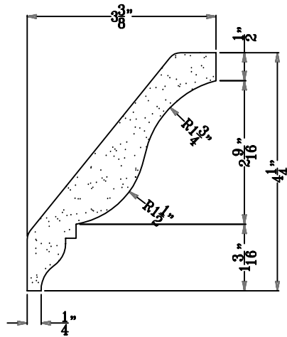
PROFILE
