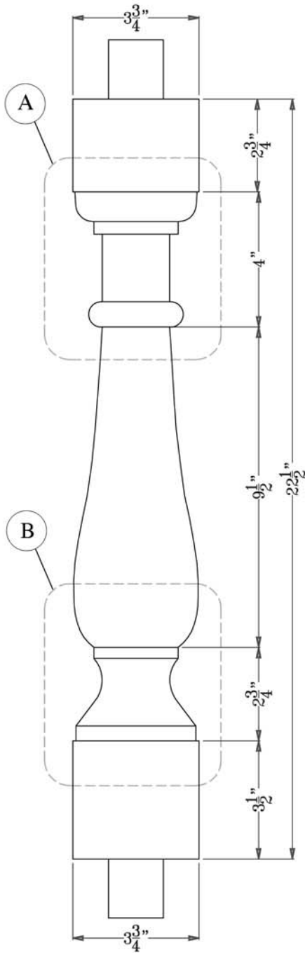
ELEVATION - BALUSTER
