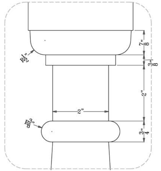
A DETAIL - BALUSTER
