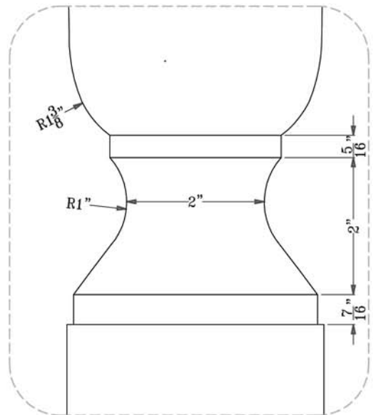
B DETAIL - BALUSTER
