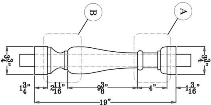
ELEVATION - BALUSTER
