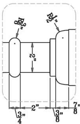
DETAIL - BALUSTER
