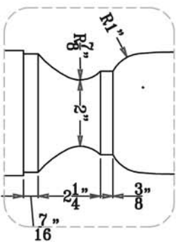
DETAIL - BALUSTER
