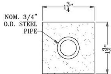
SECTION - SQ. BALUSTER
