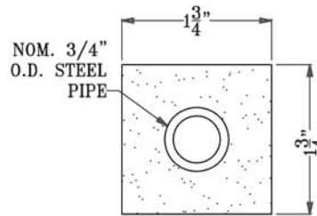
A SECTION - SQ. BALUSTER
