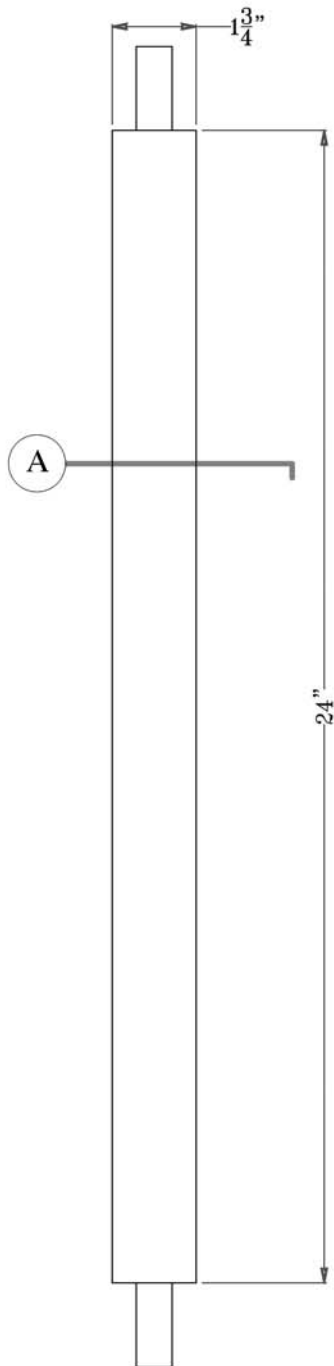
ELEVATION - SQ. BALUSTER
