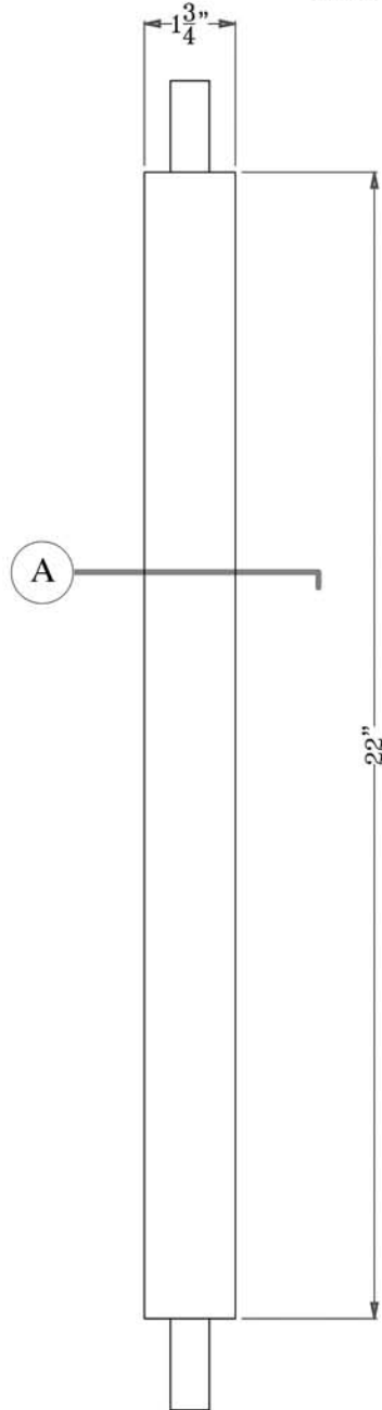
ELEVATION - SQ. BALUSTER
