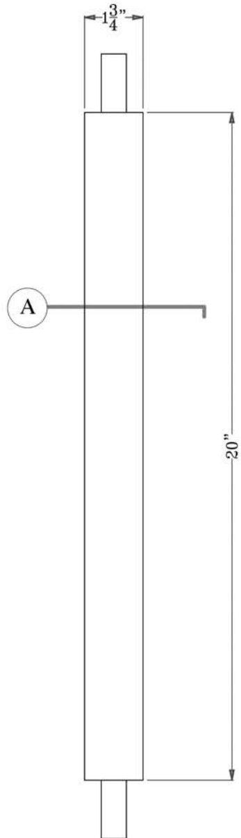
ELEVATION - SQ. BALUSTER
