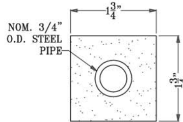
A SECTION - SQ. BALUSTER
