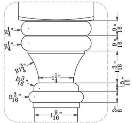
A DETAIL - BALUSTER
