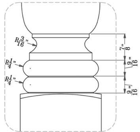
B DETAIL - BALUSTER
