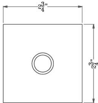
END VIEW - BALUSTER
